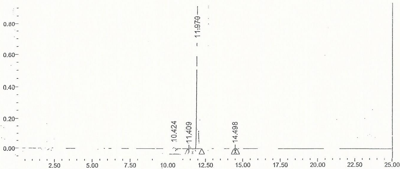
Auto-Scaled Chromatogram
